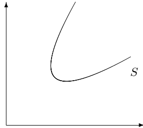
Figure 1: The hypersurface S in \mathbb{R}_{\geq 0}^n .
